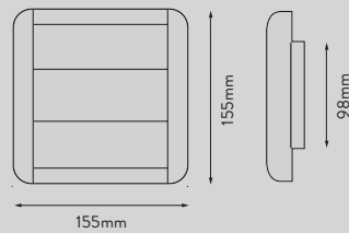
Backdraught Shutter
